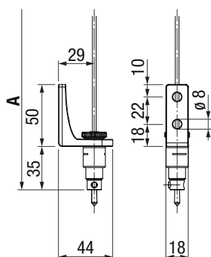
Support mural VA212-1
